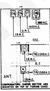
Fig. 3. R. F. Compensators Underside of Chassis
