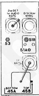
Fig. 2. I. F. Compensators Top of Chassis
